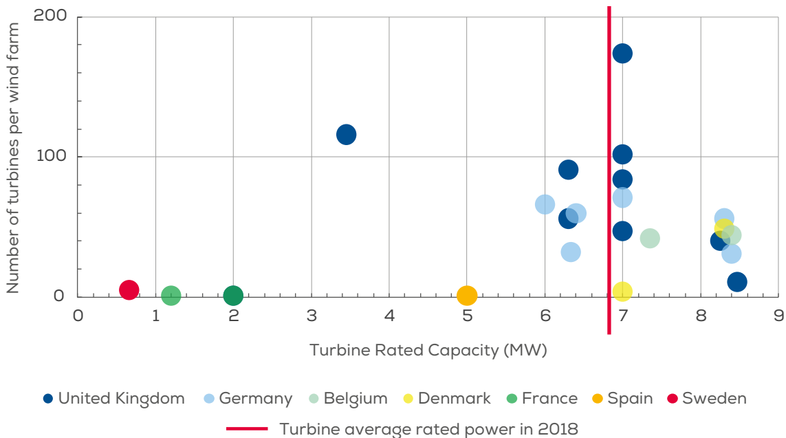
Average turbine rated capacity and number of turbines of wind farms under construction in 2018
