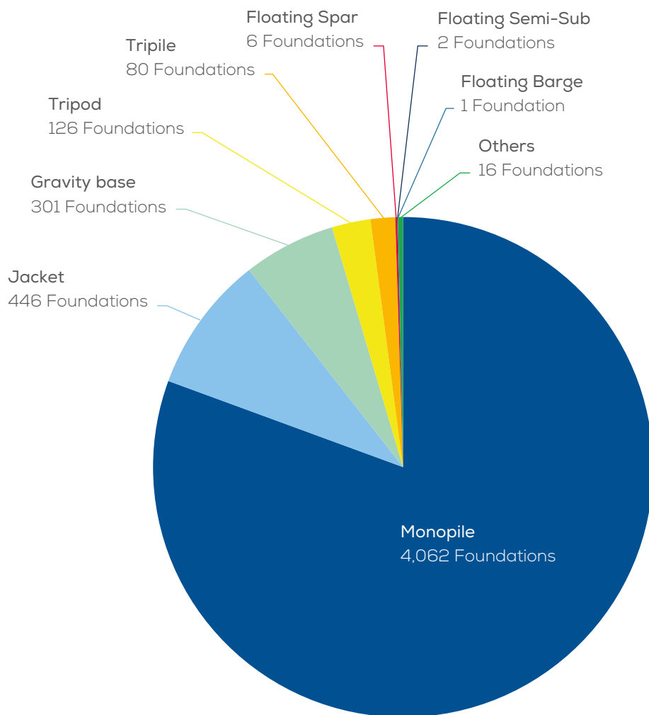
FIGURE 17 Share of substructure types for grid-connected wind turbines at the end of 2018
