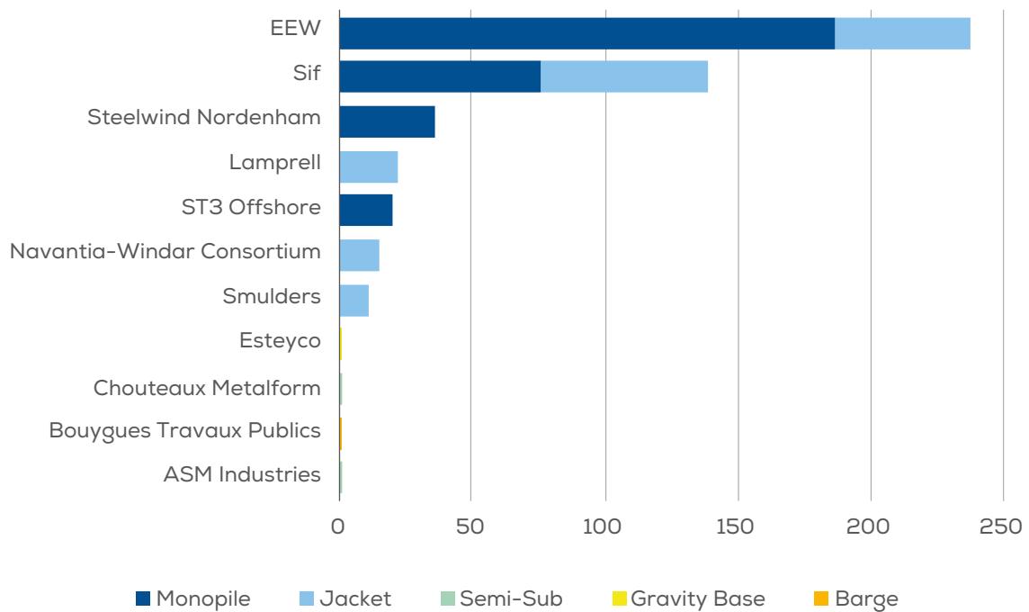
FIGURE 16 Foundations installed in 2018 by manufacturing company 7
