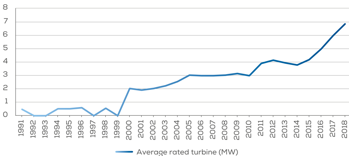
FIGURE 7 Yearly average of newly installed offshore wind turbine rated capacity (MW)
