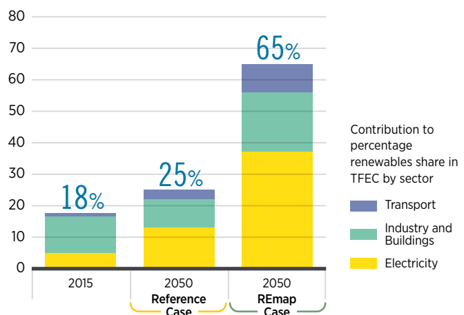
Renewables share in TFEC (%)
