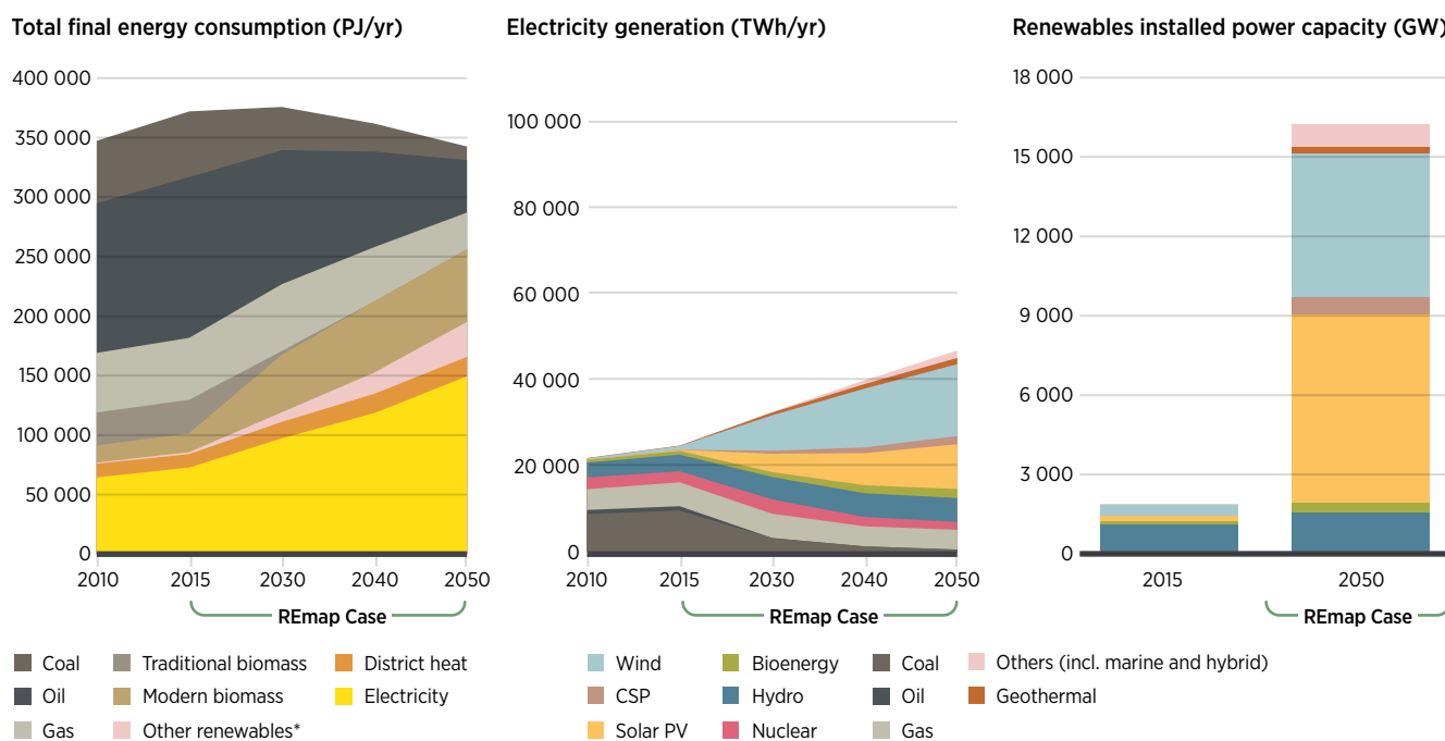
Figure 4. The rising importance of electricity derived from renewable energy Share of electricity in total final energy consumption (PJ/yr), electricity generation mix (TWh/yr), and renewable capacity developments (GW), REmap Case, 2015-2050
