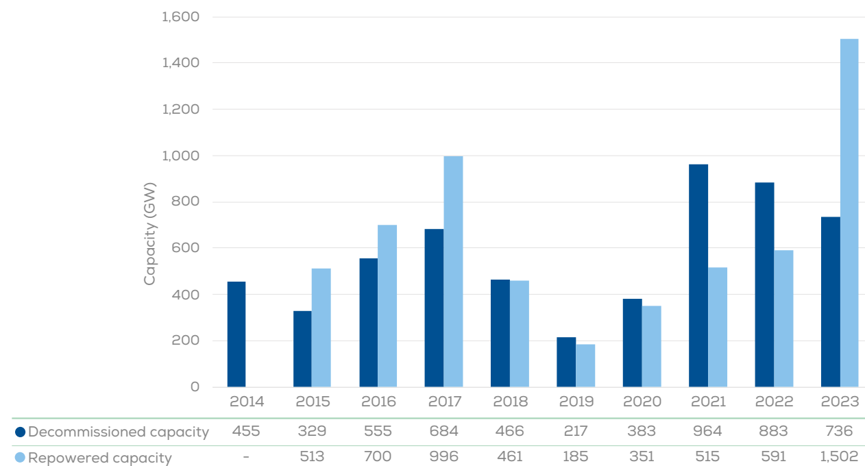
FIGURE 13. Decommissioned and repowered capacity in Europe, 2014-23
