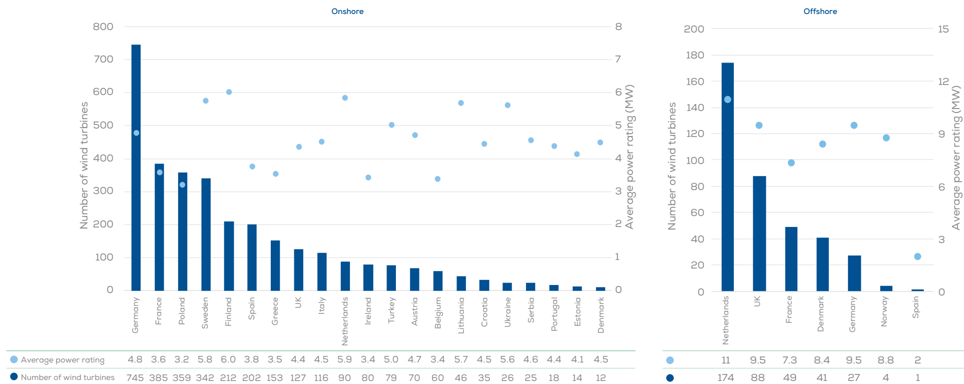
FIGURE 9. Number of turbines installed in 2023 and their average power rating
