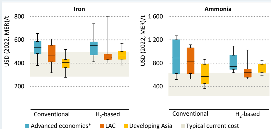
Figure 4.14 ▶ Levelised cost of production of iron and ammonia by process type in selected regions in the NZE Scenario, 2030
