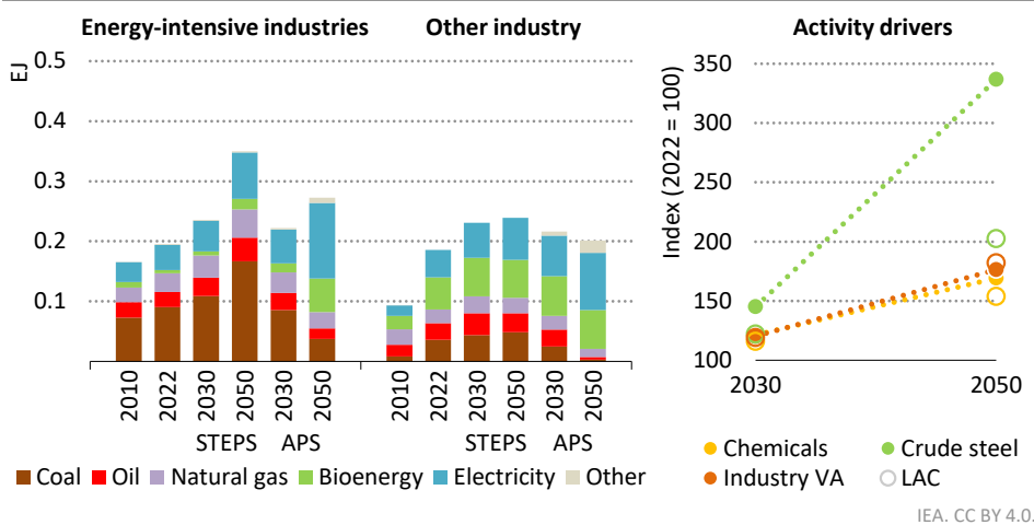
Figure 5.33 ▶ Fuel consumption in industry by type and scenario in Colombia
