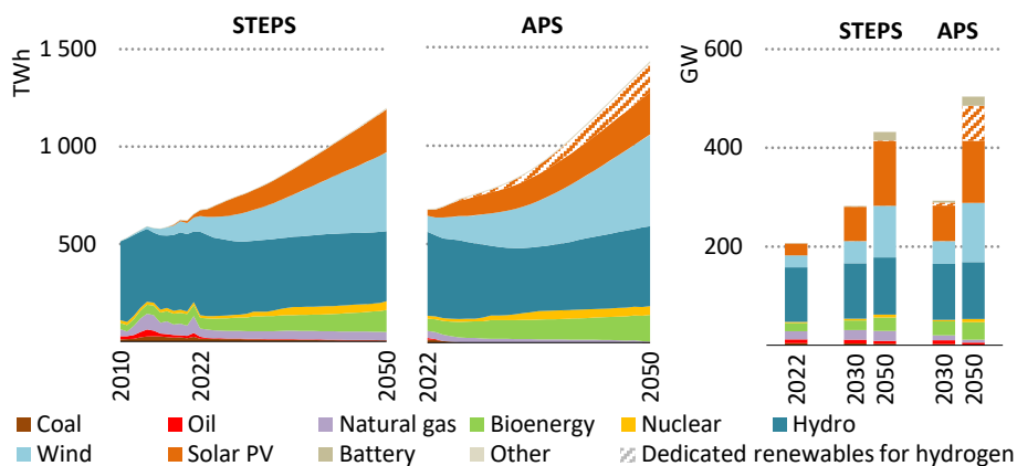
Figure 5.21 ▶ Electricity generation and capacity by fuel and scenario in Brazil
