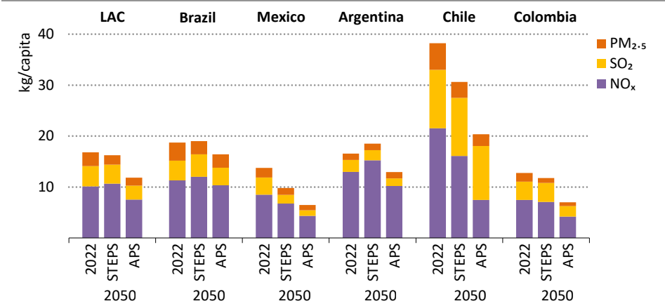
Figure 2.29 ▶ Air pollution emissions by pollutant in LAC and selected countries in 2022 and by scenario in 2050
