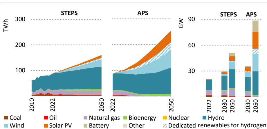
Figure 5.37 ▶ Electricity generation and capacity by fuel and scenario in Colombia
