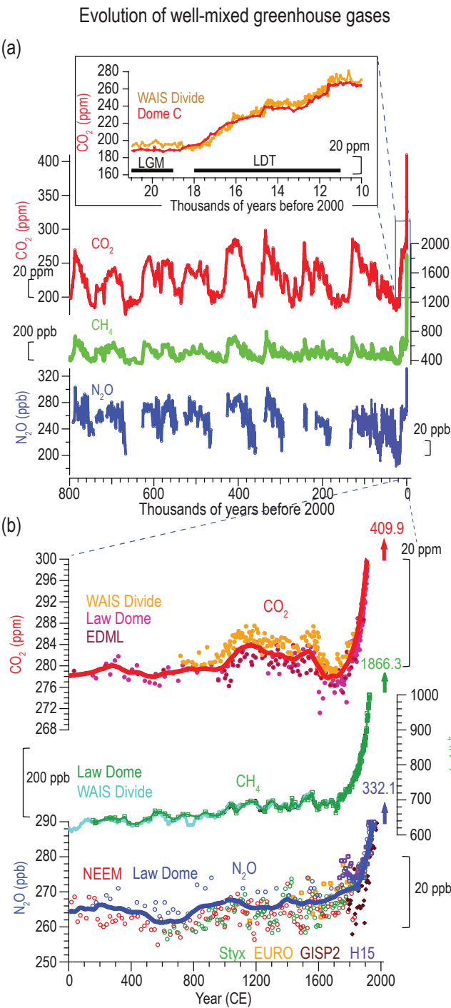
Figure 2.4 | Atmospheric well-mixed greenhouse gas (WMGHG) concentrations from ice cores. (a) Records during the last 800 kyr with the Last Glacial Maximum (LGM) to Holocene transition as inset. (b) Multiple high-resolution records over the CE. The horizontal black bars in panel (a) inset indicate LGM and Last Deglacial Termination (LDT) respectively. The red and blue lines in (b) are 100-year running averages for CO 2 and N 2 O concentrations, respectively. The numbers with vertical arrows in (b) are instrumentally measured concentrations in 2019. Further details on data sources and processing are available in the chapter data table (Table 2.SM.1).
