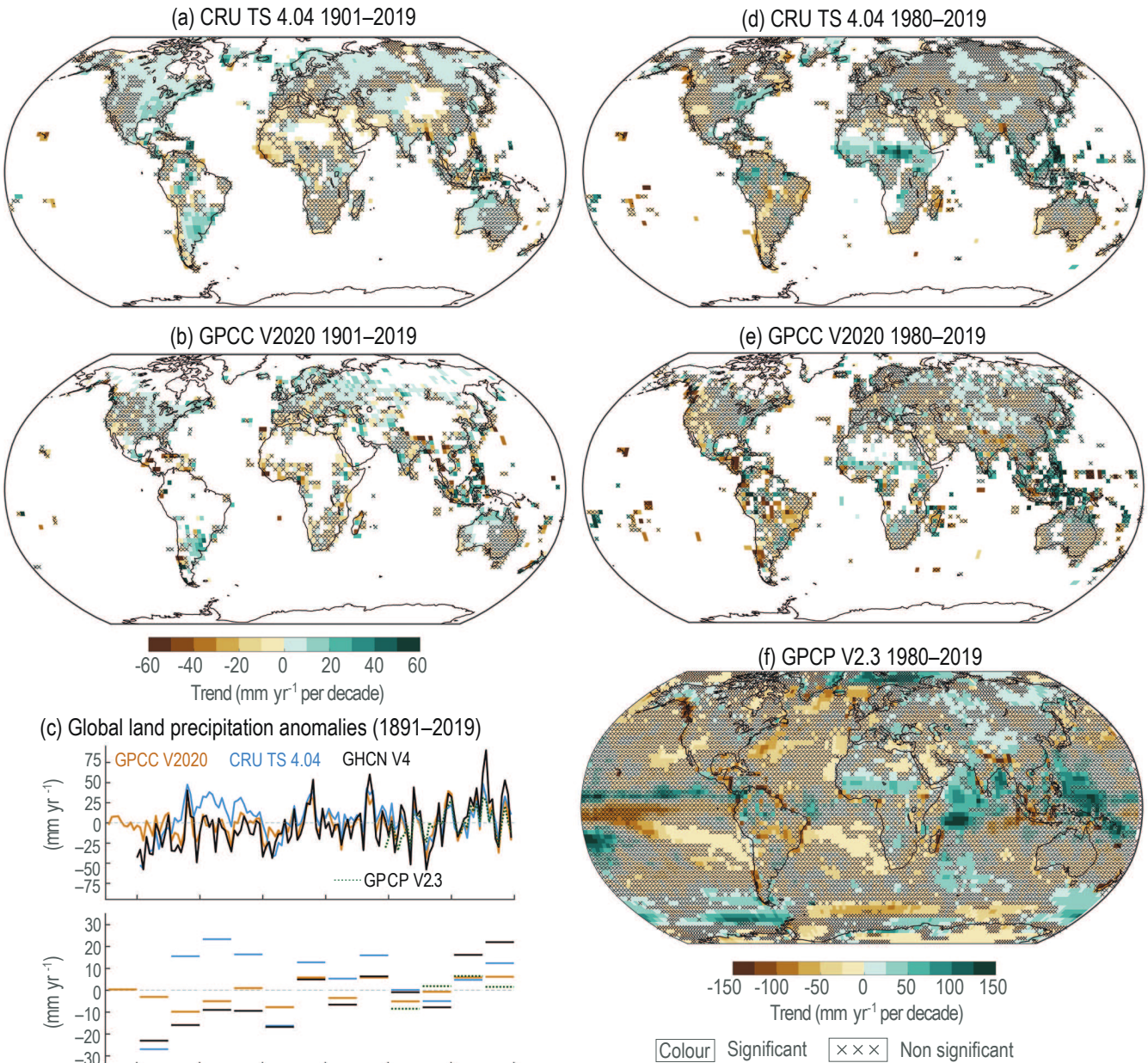
Figure 2.15 | Changes in observed precipitation. (a, b) Spatial variability of observed precipitation trends over land for 1901–2019 for two global in-situ products. Trends are calculated using OLS regression with significance assessed following AR(1) adjustment after Santer et al. (2008) ('x' marks denote non-significant trends). (c) Annual time series and decadal means from 1891 to date relative to a 1981–2010 climatology (note that different products commence at distinct times). (d, e) as (a, b), but for the periods starting in 1980. (f) is for the same period for the globally complete merged GPCP v2.3 product. Further details on data sources and processing are available in the chapter data table (Table 2.SM.1).
