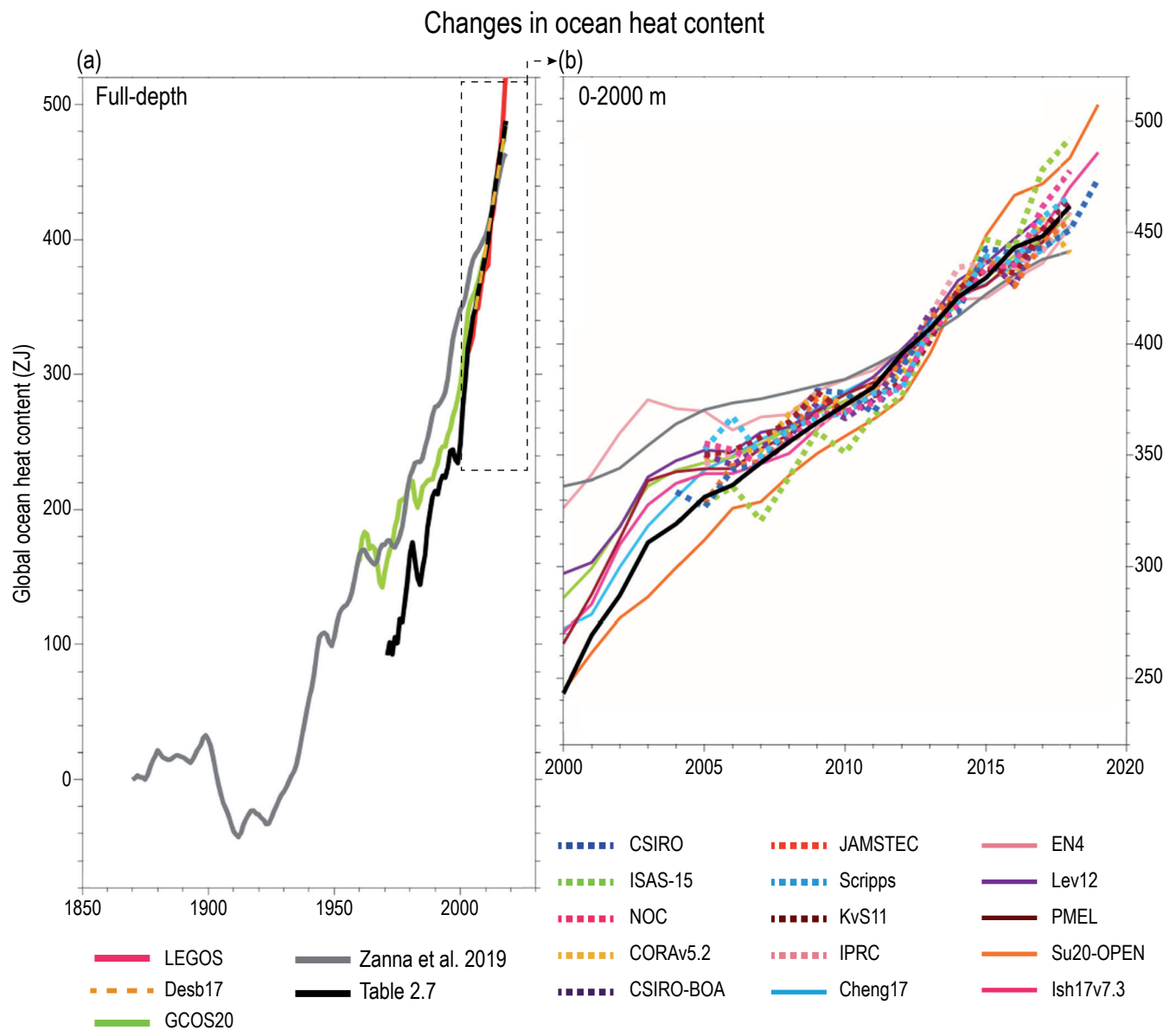
Figure 2.26 | Changes in ocean heat content (OHC). Changes are shown over (a) full depth of the ocean from 1871–2019 from a selection of indirect and direct measurement methods. The series from Table 2.7 is shown in solid black in both (a) and (b) (see Table 2.7 caption for details). (b) as (a) but for 0–2000 m depths only and reflecting the broad range of available estimates over this period. For further details see chapter data table (Table 2.SM.1).
