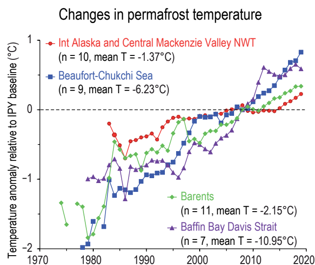
Figure 2.25 | Changes in permafrost temperature. Average departures of permafrost temperature (measured in the upper 20–30 m) from a baseline established during International Polar Year (2007–2009) for Arctic regions. Further details on data sources and processing are available in the chapter data table (Table 2.SM.1).
