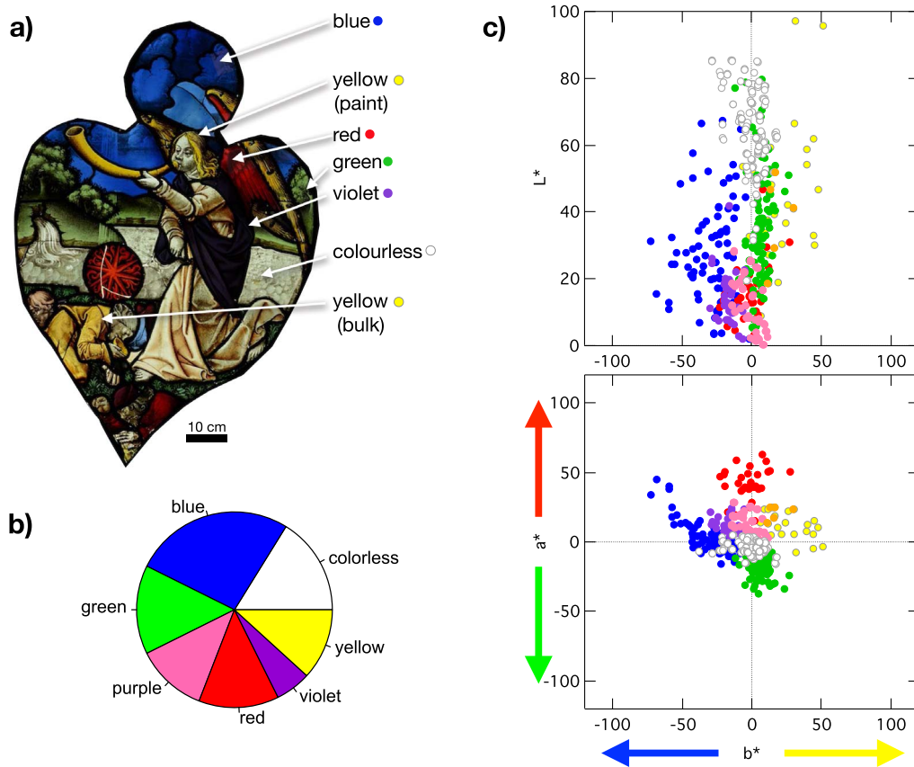
Figure 3. (a) Panel S1 and identification of the colors; (b) repartition of the analyzed colors; (c) CIE L^*a^*b^* parameters obtained from optical absorption spectroscopy.
