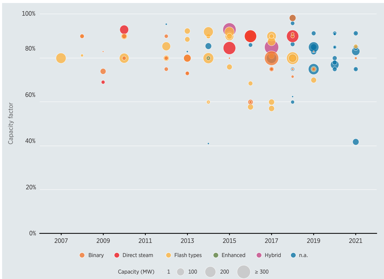
Figure 7.3 Capacity factors of geothermal power plants by technology and project size, 2007-2021
