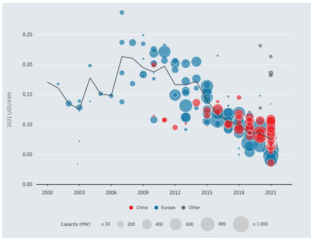
Figure 4.13 Offshore wind project and global weighted average LCOEs and auction/PPA prices, 2000-2024
