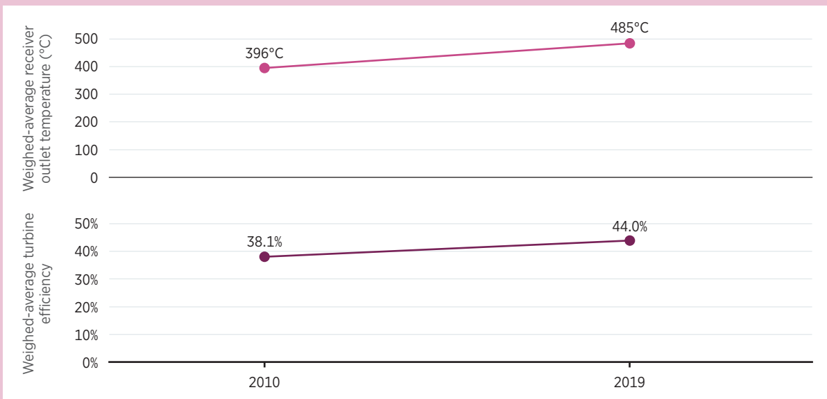
Figure B5.2 Receiver outlet temperatures and turbine efficiency trends for CSP plants (2010-2019)
