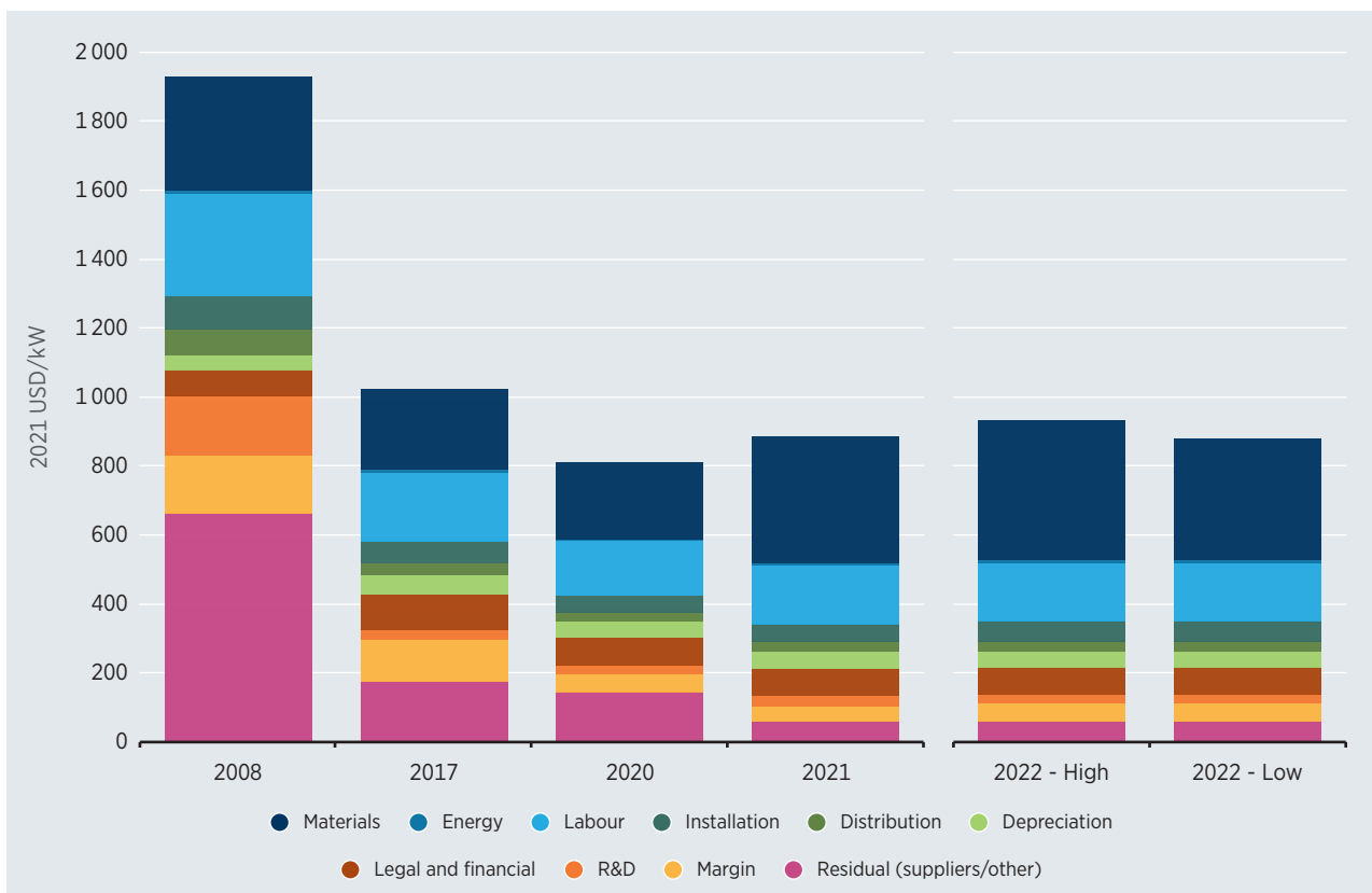
Figure 1.18 Representative wind turbine price evolution by cost component, 2008, 2017, 2020, 2021 and 2022
