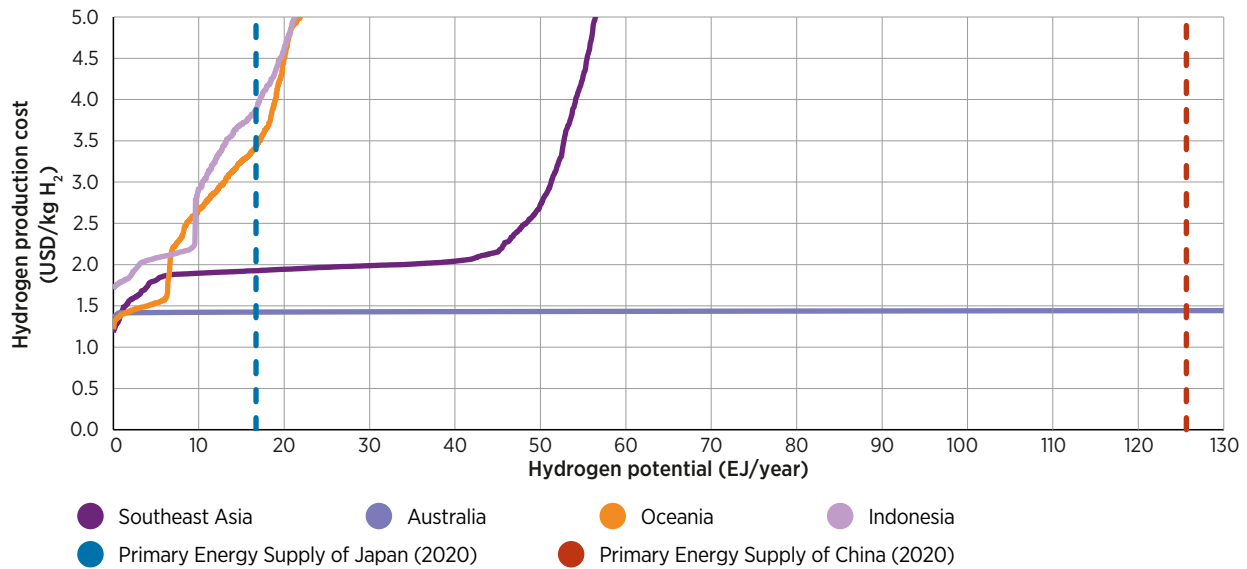
Figure 61 Hydrogen cost curve potential based on 2030 values
