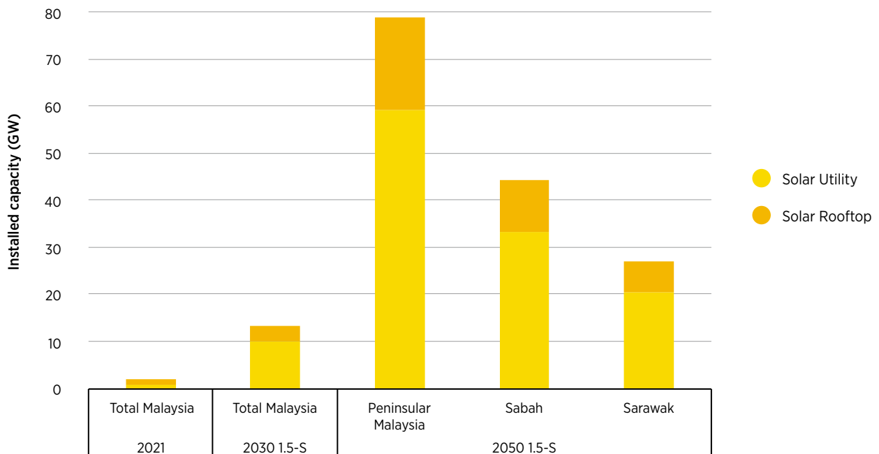
Figure 63 Solar PV installed capacity in Malaysia, 2020, 2030 and 2050
