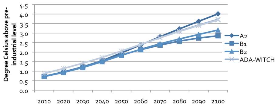
Figure 1: Temperature estimates of the IPCC SRES 1 (IIASA) , the WITCH model (Bosetti et. al 2006) and the AD-WITCH baseline scenario used in this study
